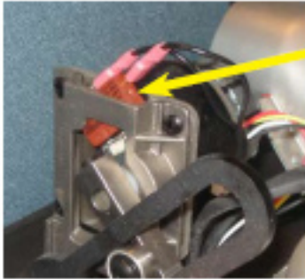
PICTURE OF THE MICRO SWITCH ON THE AUTO-CLEAN MOTOR.
